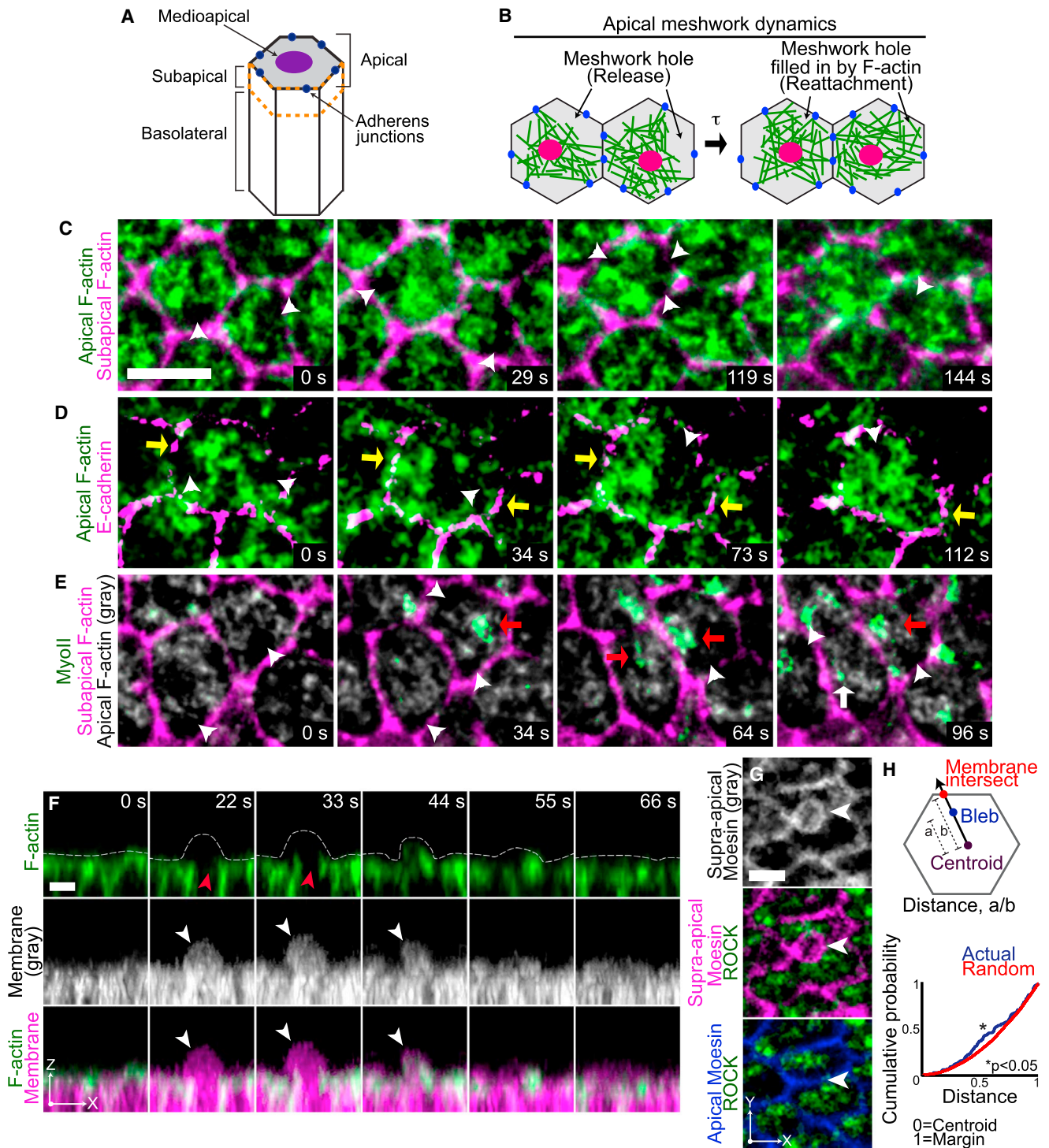
Figure 4. Medioapical Actomyosin Releases and Reattaches to AJs during Apical Constriction
