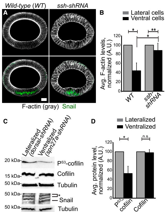
Figure 2. F-Actin Turnover Is Upregulated in Apically Constricting Cells
