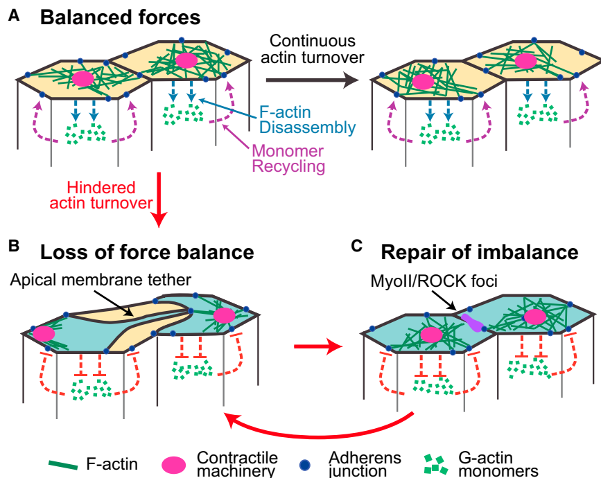
Figure 7. Model for Proper Attachment of the Contractile Machine to AJ
