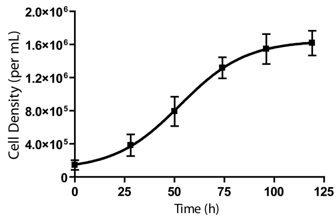
Fig. S3. Monocytic U937 cell growth in bulk. The equivalent cell density of a cell encapsulated in a 700 pL droplet is \approx 1.4 million cells/mL. The cell growth curve showed that this density is close to the plateau of the U937 growth curve. This may explain why cell growth of encapsulated cells was slow and limited to the first 24 h.
