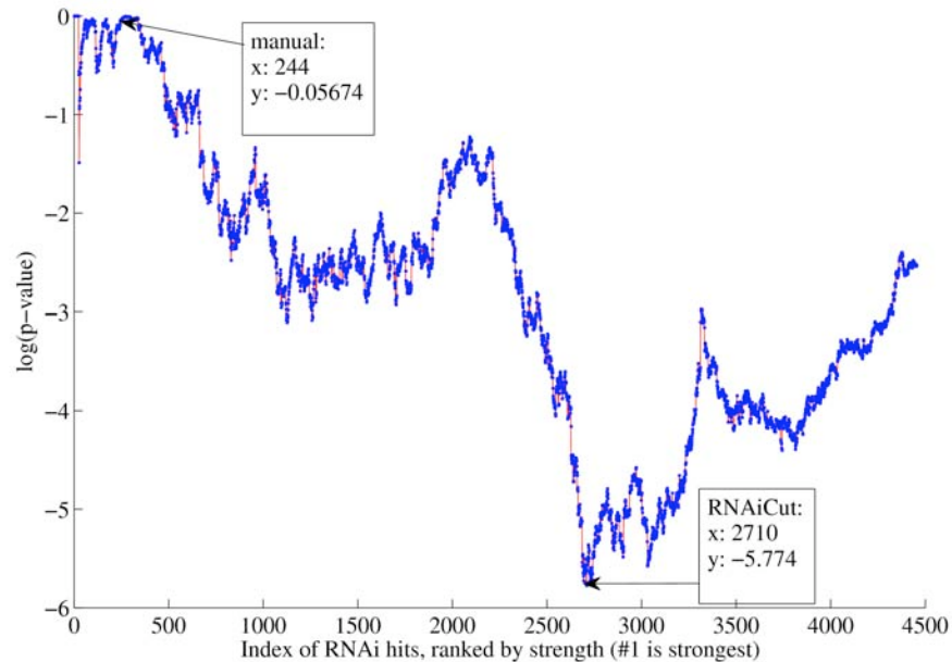
Supplementary Figure 10: Calcium entry for genes with negative scores
